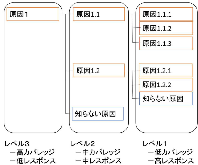
(図 13) FTA (Fault Tree Analysis) 及び 階層化 FDIR (Fault Detection, Isolation and Recovery)
